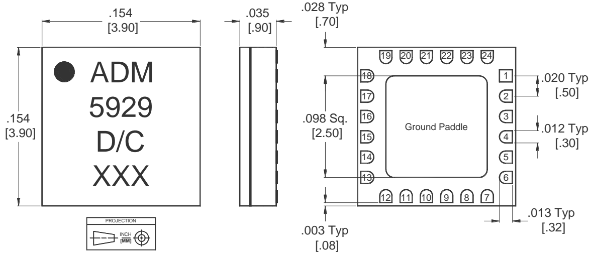
Outline Drawing
