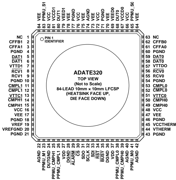
Figure 8. Pin Configuration
