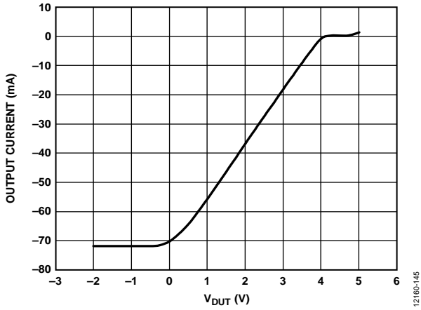
Figure 45. Reflection Clamp Current Limit, VCHx = 5.0 V, VCLx = 4.0 V; V DUTx Swept from -2.0 V to +5.0 V
