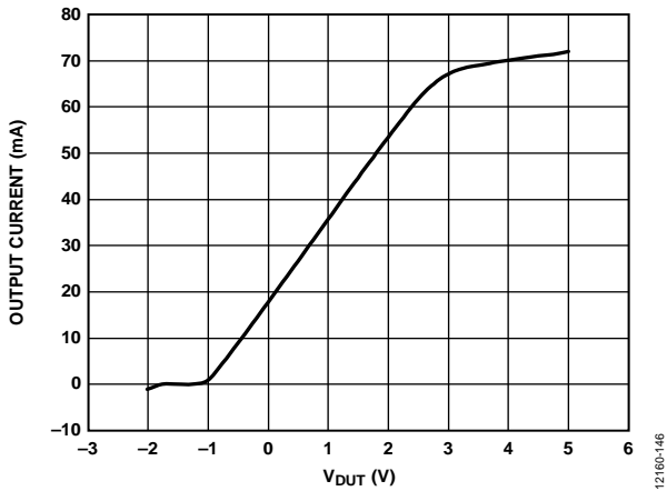
Figure 46. Reflection Clamp Current Limit, VCHx = -1.0 V, VCLx = -2.0 V; V DUTx Swept from -2.0 V to +5.0 V
