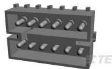
TE 系列/零件编号350220-1 12P CMNL HDR ASSY PC NATL
