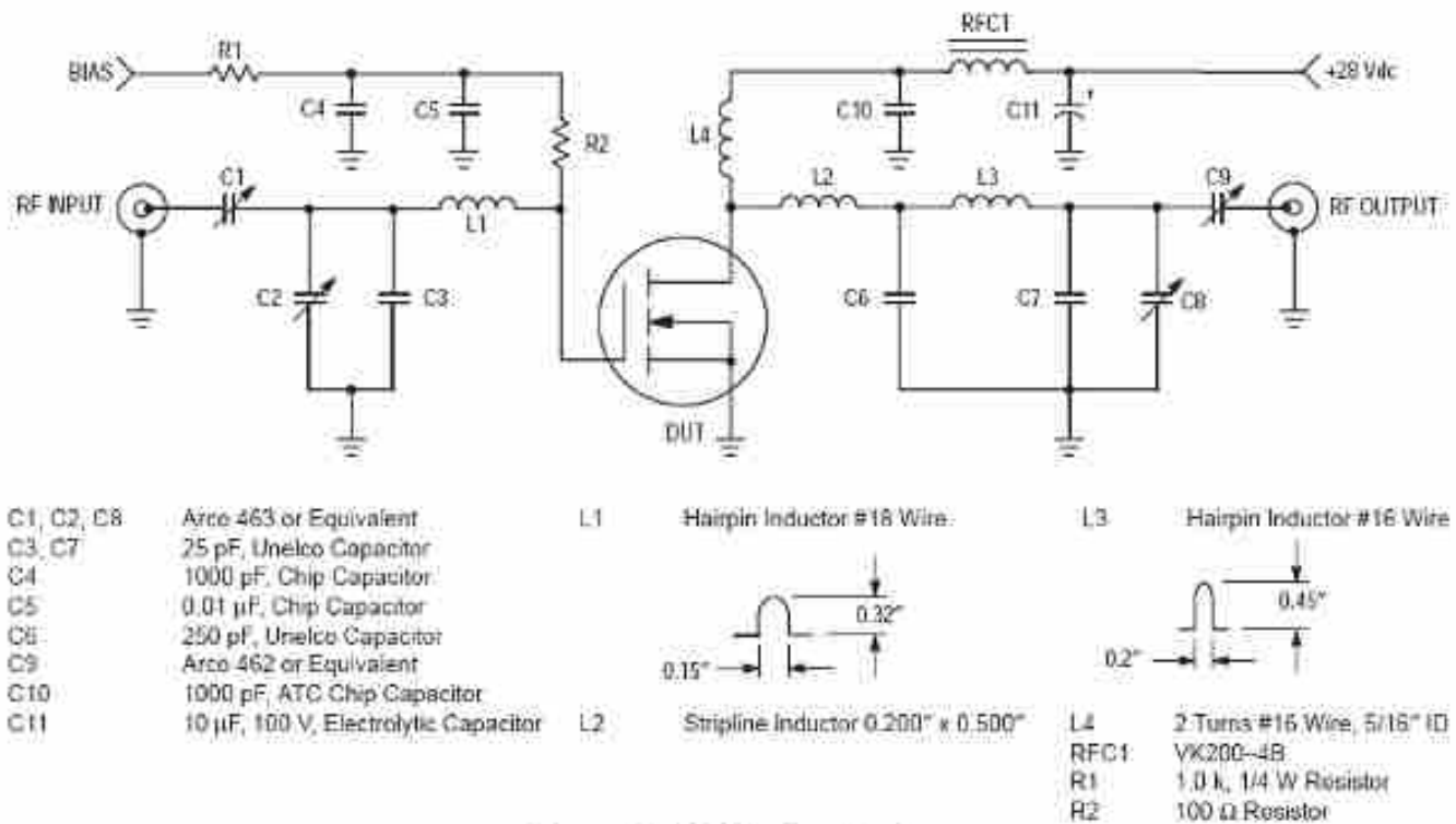
Figure 11. 225 MHz Test Circuit
