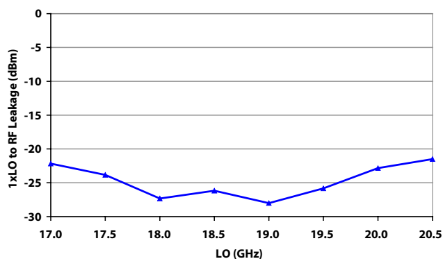
XU1006-QB, 1xLO to RF Leakage (dBm), P LO =+2dBm
