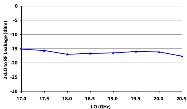
XU1006-QB, 2xLO to RF Leakage (dBm), P LO =+2dBm
