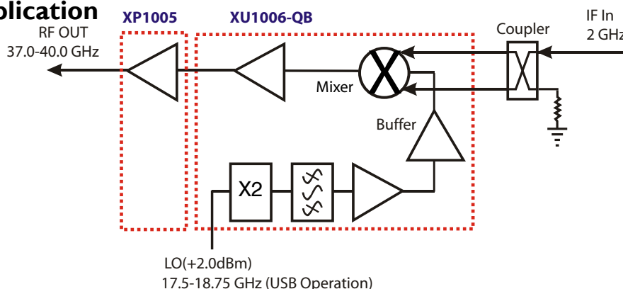
Mimix Broadband MMIC-based 37.0-40.0 GHz Transmitter Block Diagram
