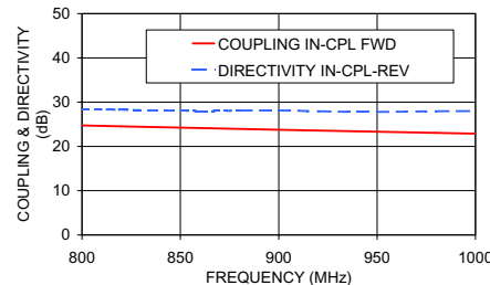
SYBD-23-13HP+ COUPLING & DIRECTIVITY
