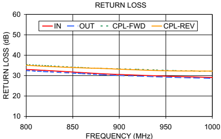
SYBD-20-13HP+ RETURN LOSS
