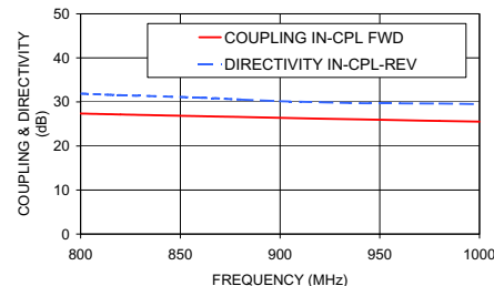
SYBD-26-13HP+ COUPLING & DIRECTIVITY
