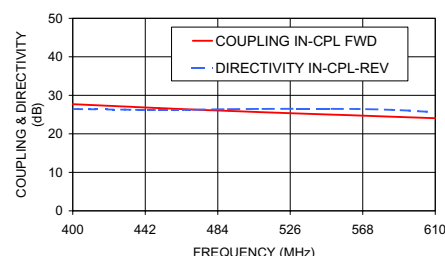
SYBD-26-62HP+ COUPLING & DIRECTIVITY
