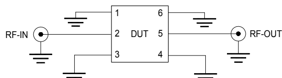
Fig 1. Block diagram of Test Circuit used for characterization, Test board TB-934-20C+ Conditions: Attenuation, VSWR: Pin=0 dBm
