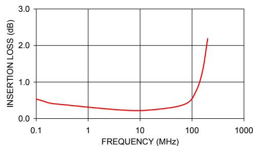
TMO-4-6+ INSERTION LOSS
