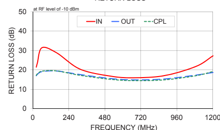
LRDC-10-2W-75J+ RETURN LOSS
