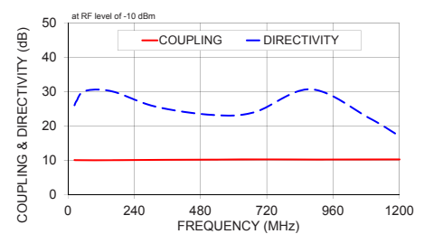
LRDC-10-2W-75J+ COUPLING & DIRECTIVITY
