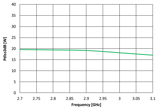
Pdiss3dB At 25 °C
