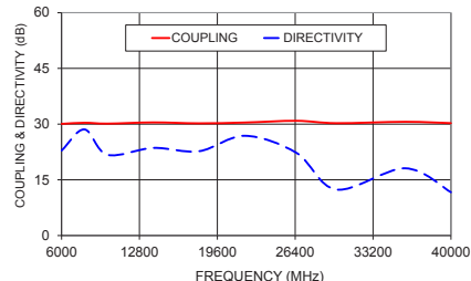
ZCDC30-K0644+ COUPLING & DIRECTIVITY
