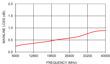
ZCDC30-K0644+ MAINLINE LOSS
