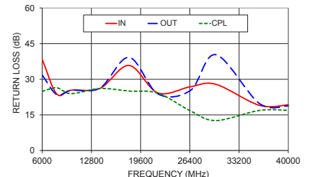
ZCDC30-K0644+ RETURN LOSS
