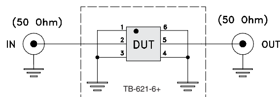
Fig 1. Block diagram of Test Circuit used for characterization, Test board TB-621-6+ Conditions: Attenuation, VSWR: Pin=-10 dBm
