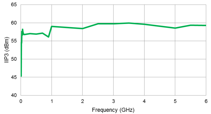
Input IP3 vs. Frequency Temp = +25°C
