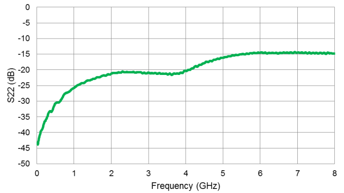
RFX (Terminated) Return Loss vs. Frequency, Temp. = +25°C
