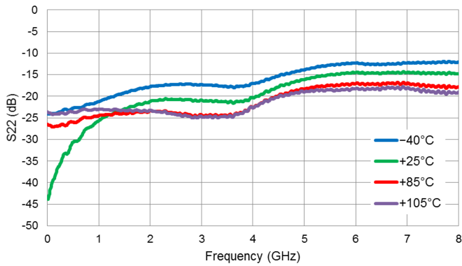
RFX (Terminated) Return Loss vs. Frequency
