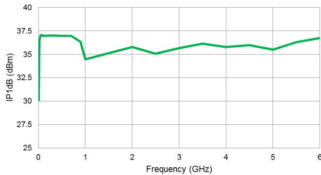
Input P1dB vs. Frequency Temp. = +25°C
