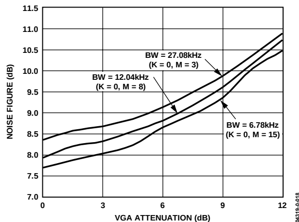
Figure 18. Noise Figure vs. VGA Attenuation ( f_{CLK} = 13\text{ MSPS} )
