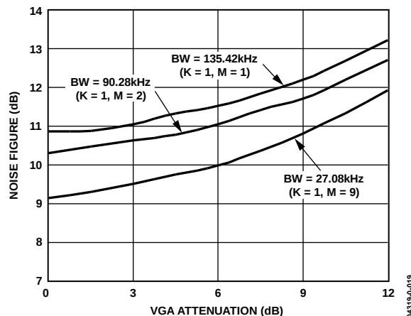
Figure 19. Noise Figure vs. VGA Attenuation ( f_{CLK} = 26\text{ MSPS} )
