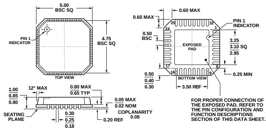
Figure 62. 32-Lead Lead Frame Chip Scale Package [LFCSP_VQ] 5 mm x 5 mm Body, Very Thin Quad (CP-32-2) Dimensions shown in millimeters
