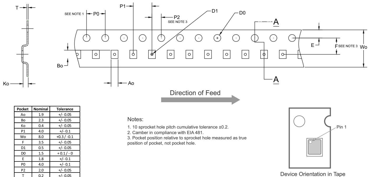
Figure 11 ■ Tape and Reel Specifications for the PE29101.
