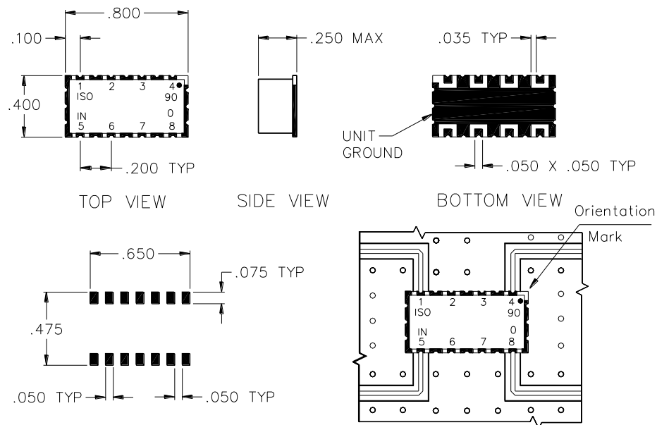
Board Installation Pattern
