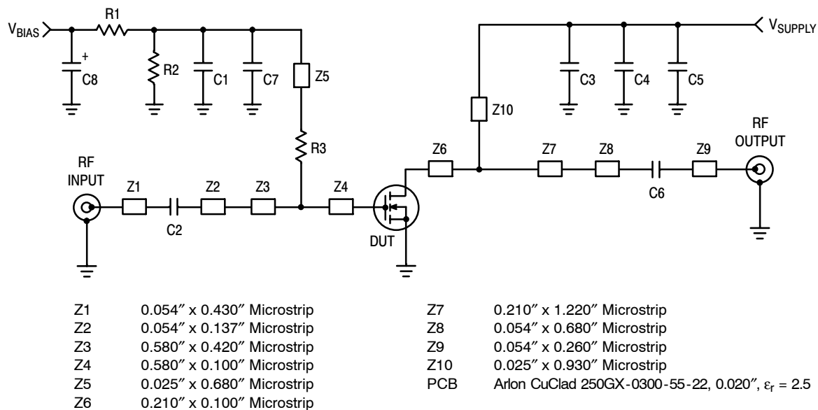
Figure 1. MW6S004NT1 Test Circuit Schematic
