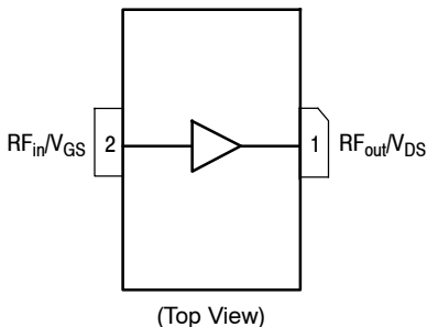
Figure 1. Pin Connections
