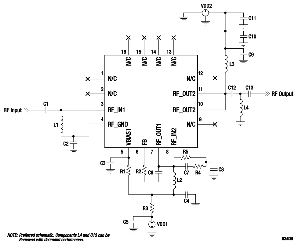
Figure 16. SKY67105-306LF Evaluation Board Schematic (For 850 MHz and V_{DD} = +5\text{ V} )
