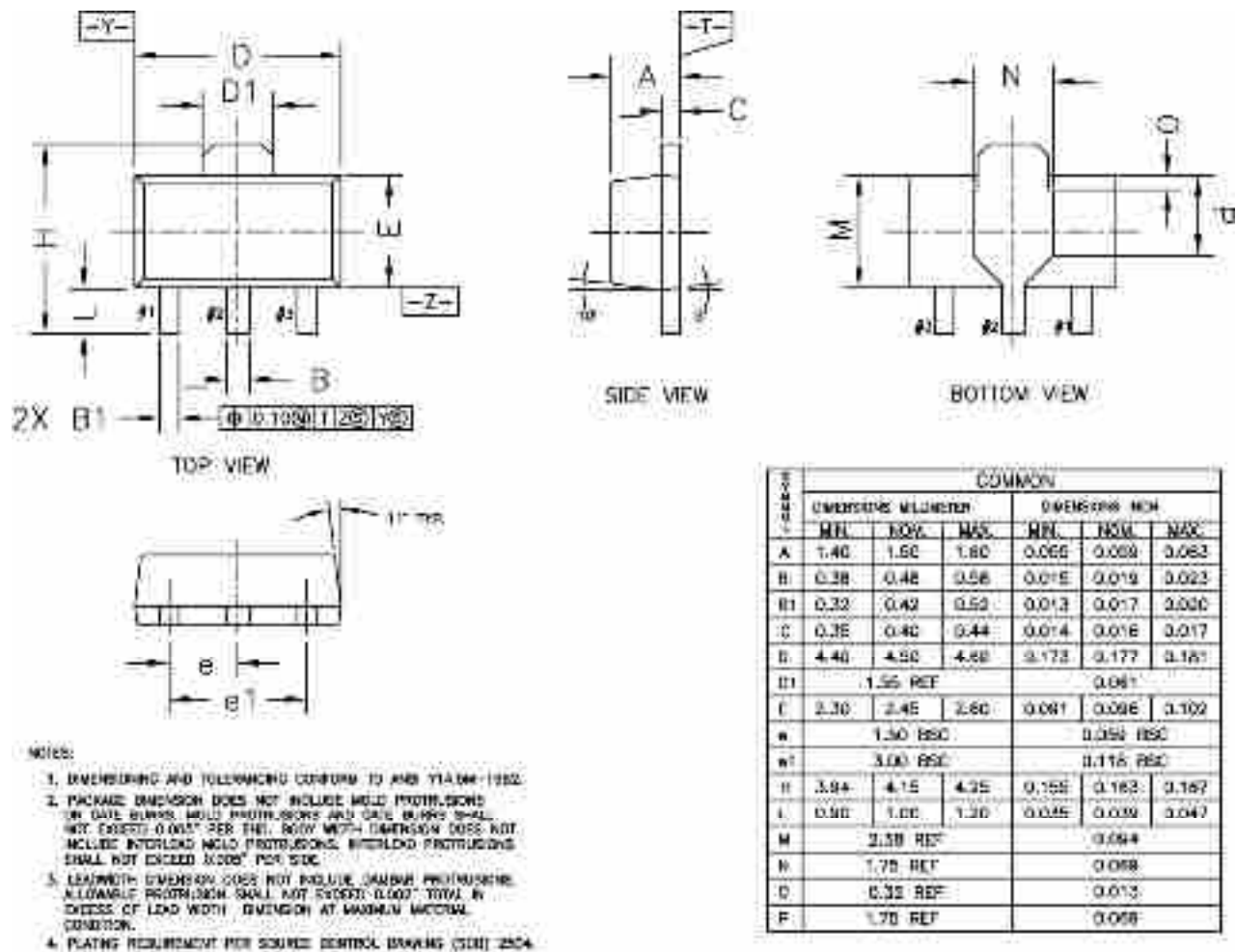
Figure 99. SKY65009 SOT-89 Package Dimensions
