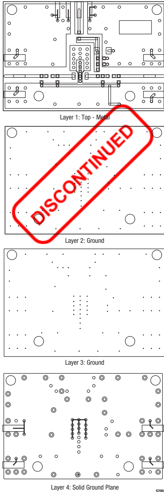
Figure 95. Evaluation Board Layer Detail
