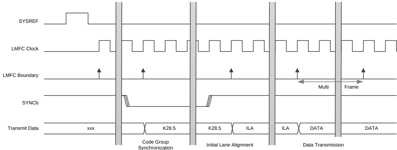
图 67. ILA Sequence
