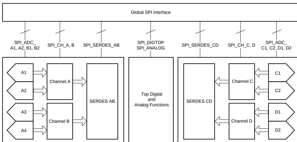
图 76. SPI Register Block Diagram
