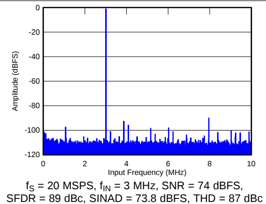
Figure 141. FFT for 20-MSPS Sampling Speed
