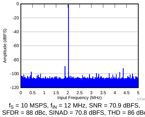
Figure 118. FFT for 10-MSPS Sampling Speed
