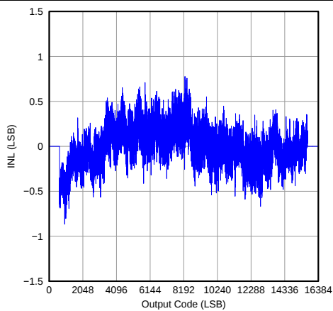
Figure 61. Integral Nonlinearity
