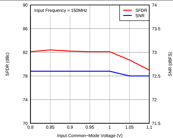
Figure 74. Performance vs Input Common-Mode Voltage
