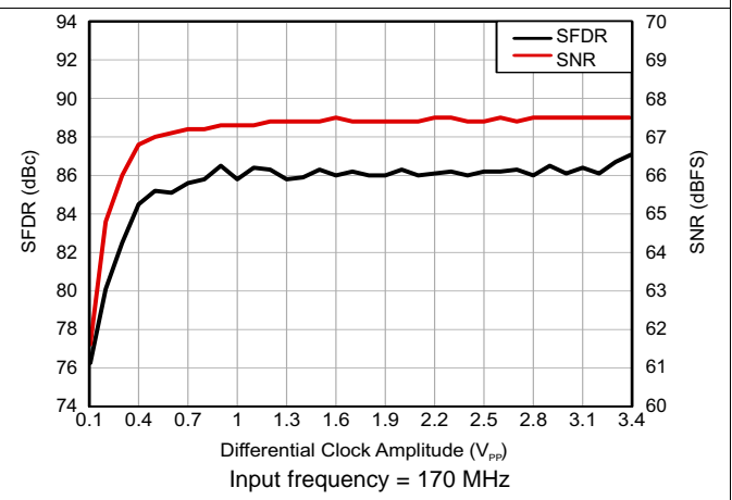
Figure 34. Performance Across Input Clock Amplitude
