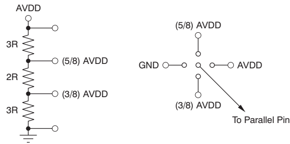
Figure 65. Simplified Diagram to Configure the DFS Pin
