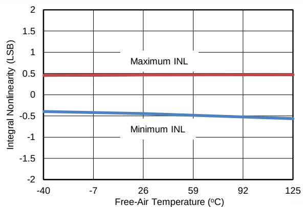
Figure 18. Typical INL
