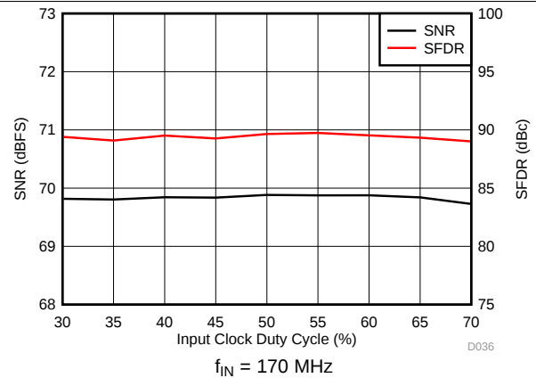
Figure 42. Performance vs Clock Duty Cycle
