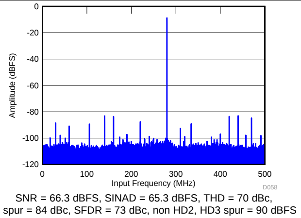
Figure 10. FFT for 720-MHz Input Signal at -6\text{ dBFS}
