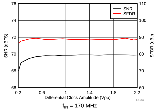
Figure 40. Performance vs Sampling Clock Amplitude
