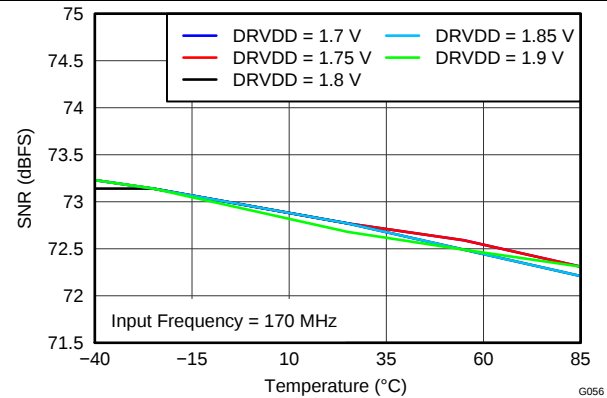
Figure 56. SNR vs DRVDD Supply and Temperature (170 MHz)
