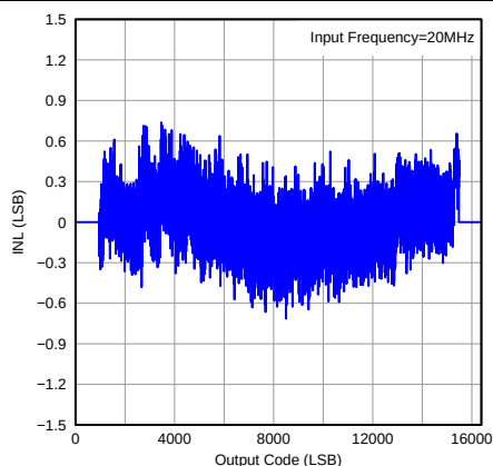
图 46. Integrated Nonlinearity
