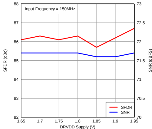
图 43. Performance vs DRVDD Supply Voltage
