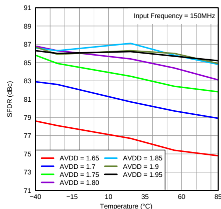
图 41. SFDR vs Temperature and AVDD Supply
