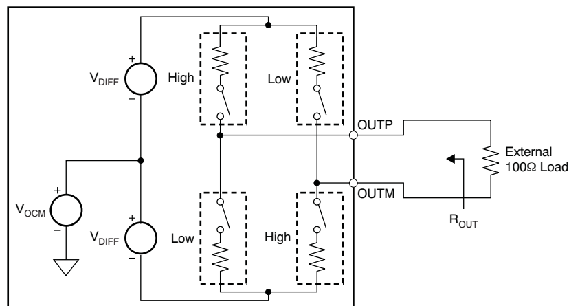
图 156. LVDS Buffer Equivalent Circuit
