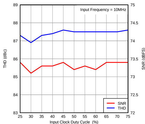
图 45. Performance vs Input Clock Duty Cycle
