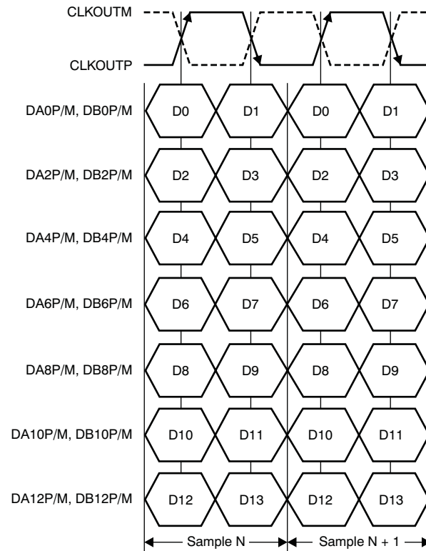
图 155. DDR LVDS Interface Timing
