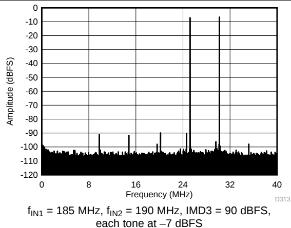
Figure 79. FFT FOR Two-Tone Input Signal ( -7\text{ dBFS} at 185 MHz and 190 MHz)
