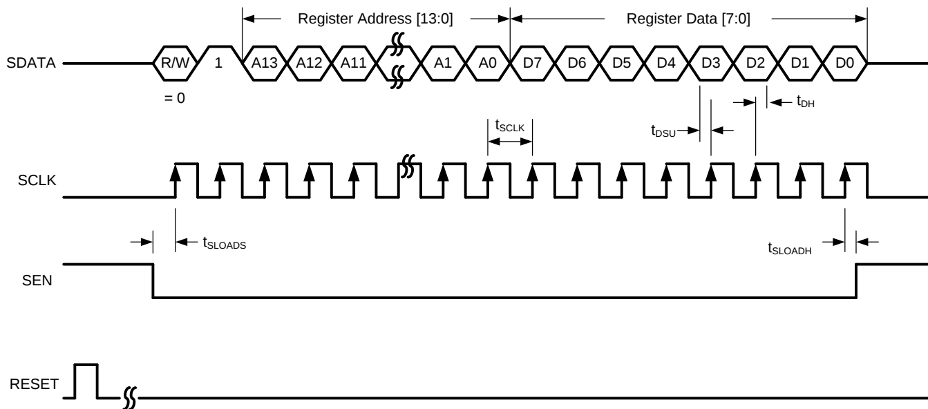
Figure 157. Serial Register Write Timing Diagram
