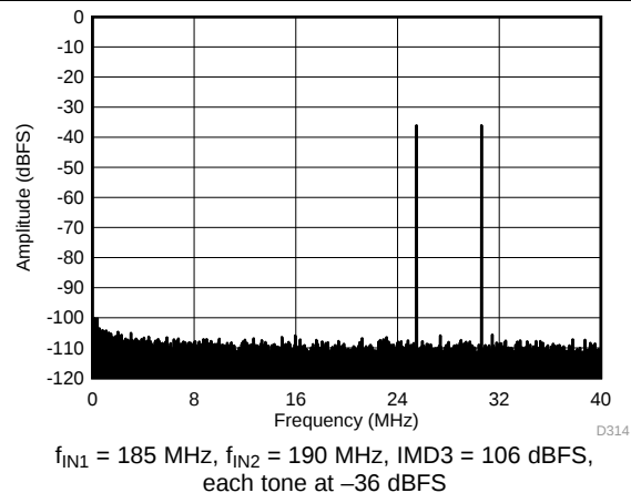
Figure 80. FFT FOR Two-Tone Input Signal ( -36\text{ dBFS} at 185 MHz and 190 MHz)
