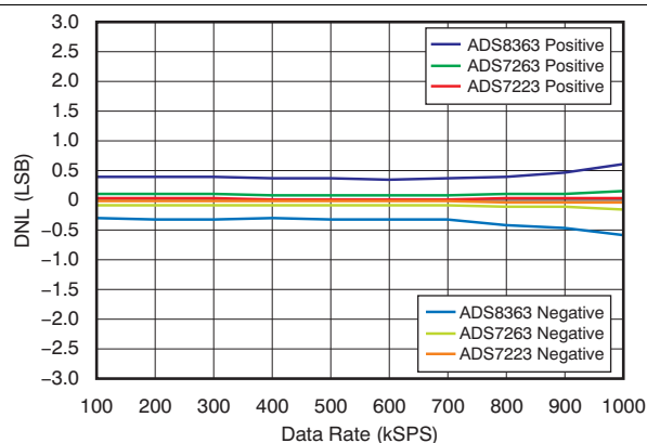
Figure 4. Differential Nonlinearity vs Data Rate
