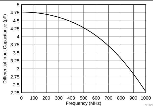
Figure 135. C_{IN} vs Input Frequency
