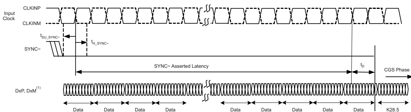
Figure 144. SYNC~ Latency in CGS Phase (Two-Lane Mode)
