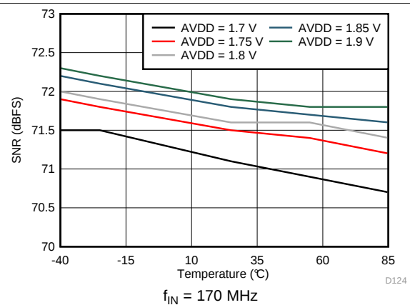
图 24. Signal-to-Noise Ratio vs AVDD Supply and Temperature
