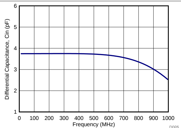
Figure 177. Differential Input Capacitance (C IN )
