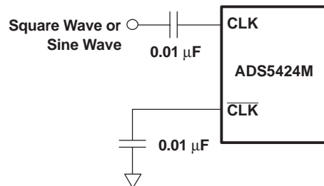
Figure 21. Single-Ended Clock
