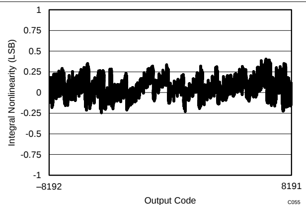
Figure 45. Typical INL
