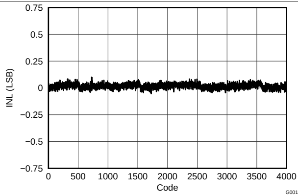
Figure 4. Integral Nonlinearity vs Code (ADS8528)
