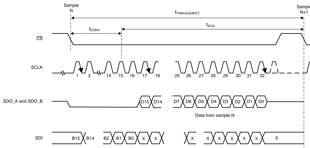
图 25. 32-CLK, Dual-SDO Mode Timing Diagram
