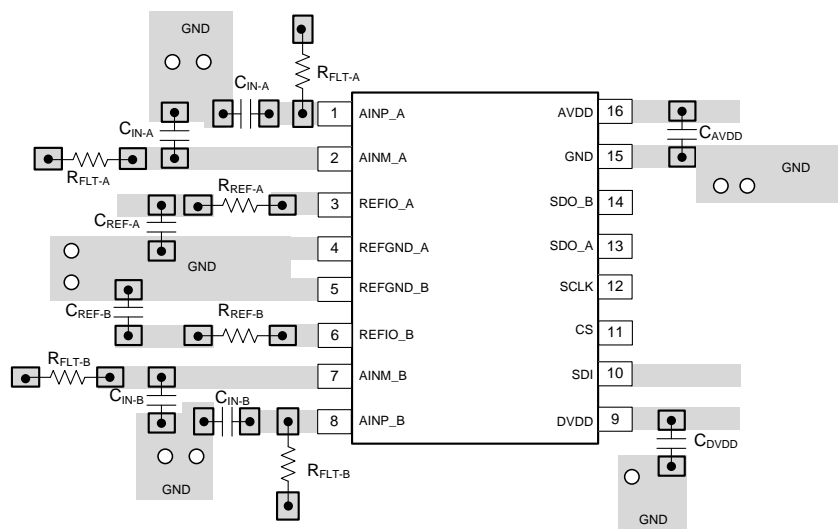
图 39. Recommended Layout
