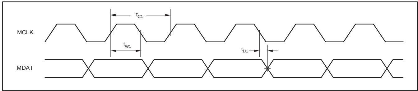
Figure 1. Mode 0 Operation
