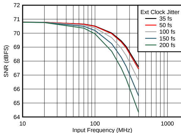
Figure 137. SNR vs Frequency for Different Clock Jitter
