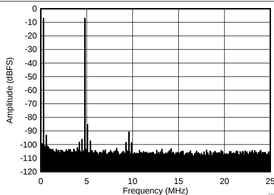
Figure 39. FFT for 450-MHz Input Signal (Dither On)
