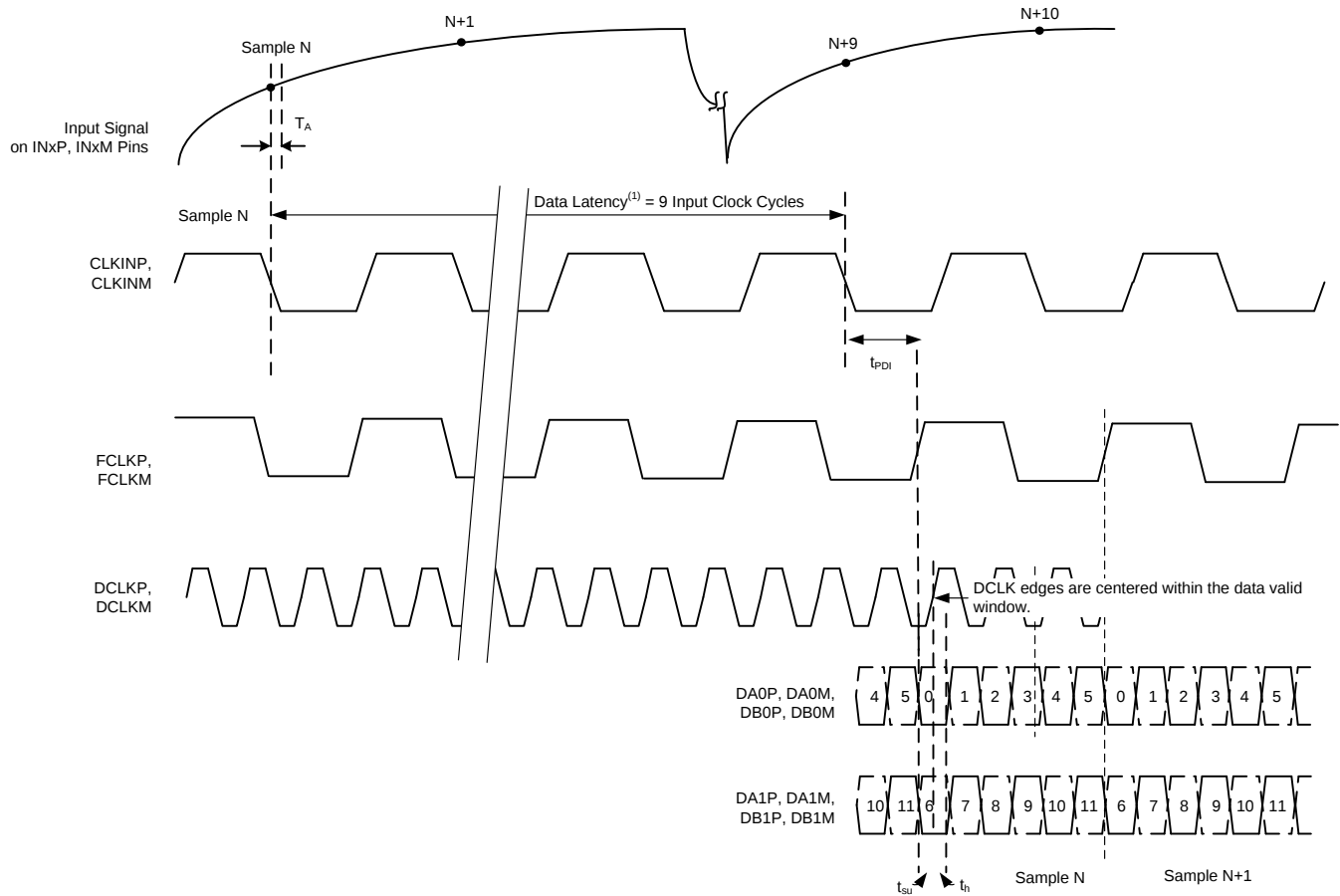
Figure 131. Latency Diagram
