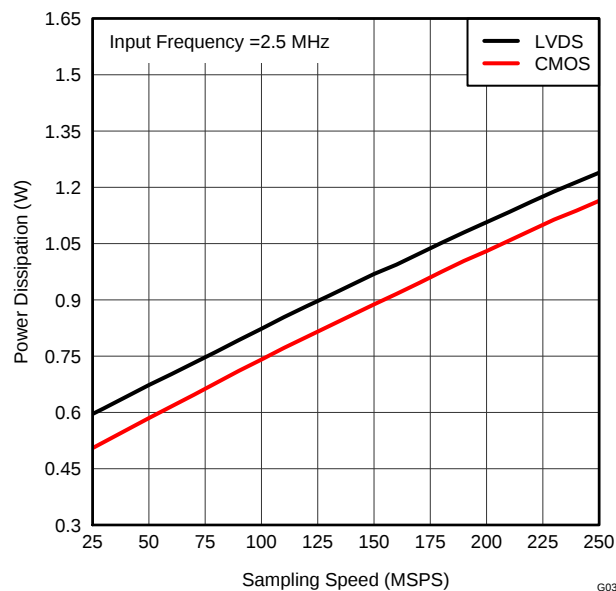
Figure 30. POWER DISSIPATION vs SAMPLING FREQUENCY
