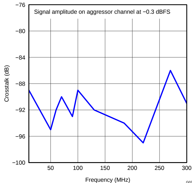
Figure 28. CROSSTALK vs FREQUENCY
