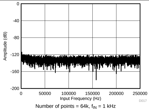
Figure 34. Typical FFT Plot (All Ranges) for the ADS8675
