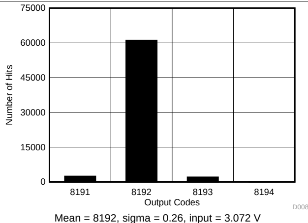
Figure 20. DC Histogram for Mid-Scale Inputs (0 V–6.144 V)
