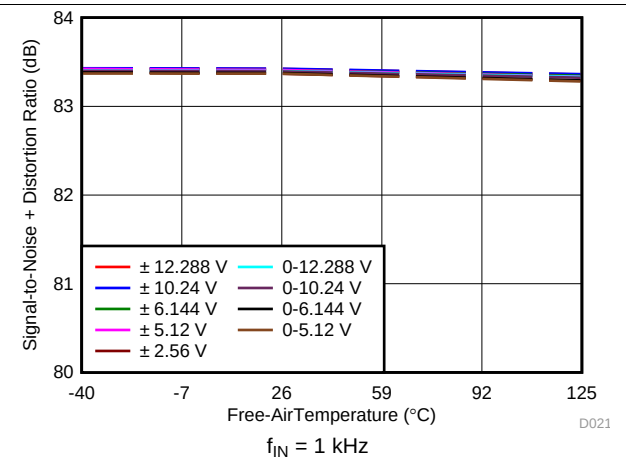
Figure 38. SINAD vs Temperature
