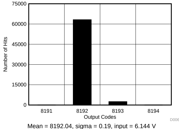
Figure 18. DC Histogram for Mid-Scale Inputs (0 V–12.288 V)
