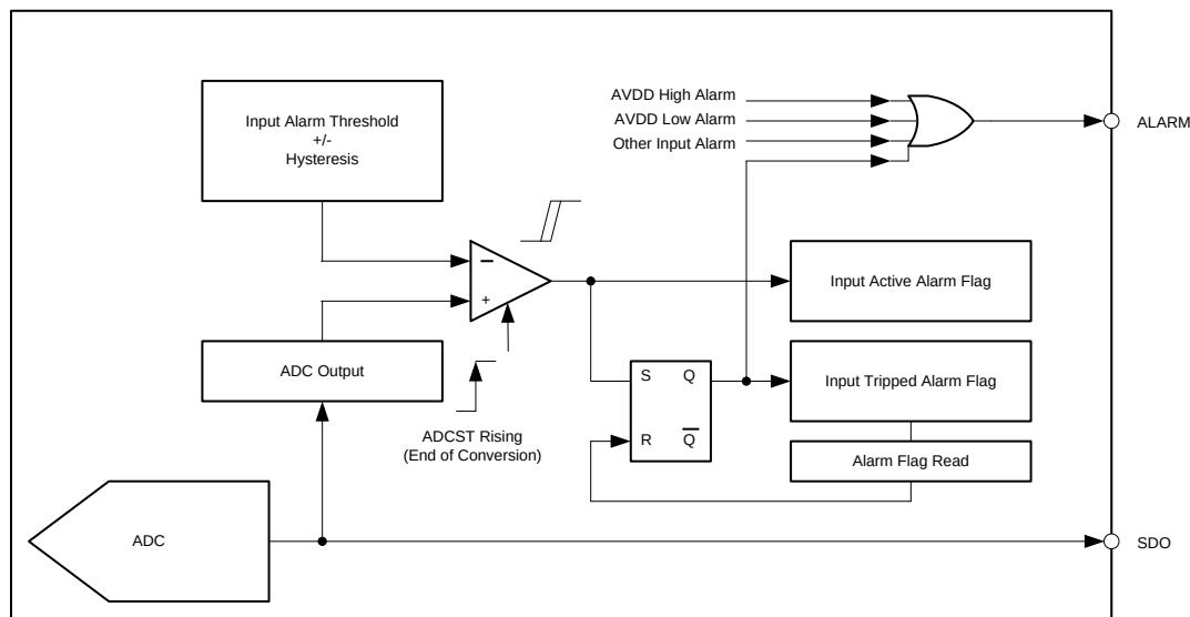
Figure 61. Alarm Functionality Schematic
