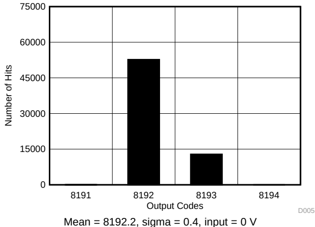
Figure 17. DC Histogram for Mid-Scale Inputs ( \pm 2.56\text{ V} )
