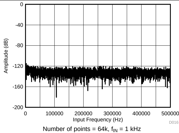
Figure 33. Typical FFT Plot (All Ranges) for the ADS8671
