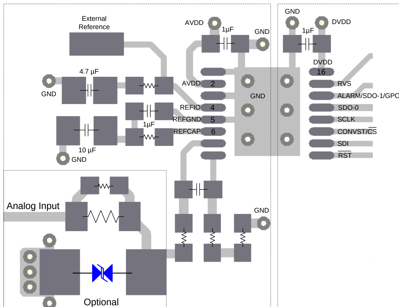
Figure 95. Board Layout for the ADS867x
