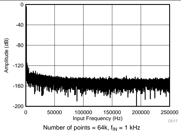
Figure 34. Typical FFT Plot (All Ranges) for the ADS8695
