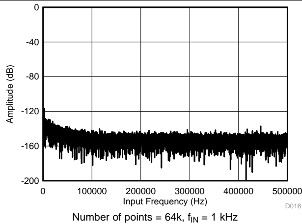
Figure 33. Typical FFT Plot (All Ranges) for the ADS8691
