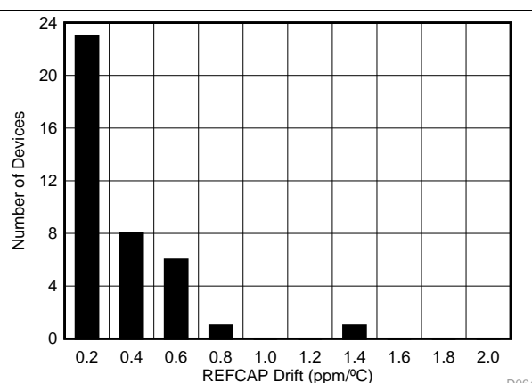
Figure 60. Reference Buffer Temperature Drift Histogram
