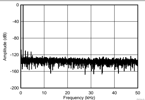
Figure 92. FFT Plot With an AC Common-Mode at 500 kSPS
