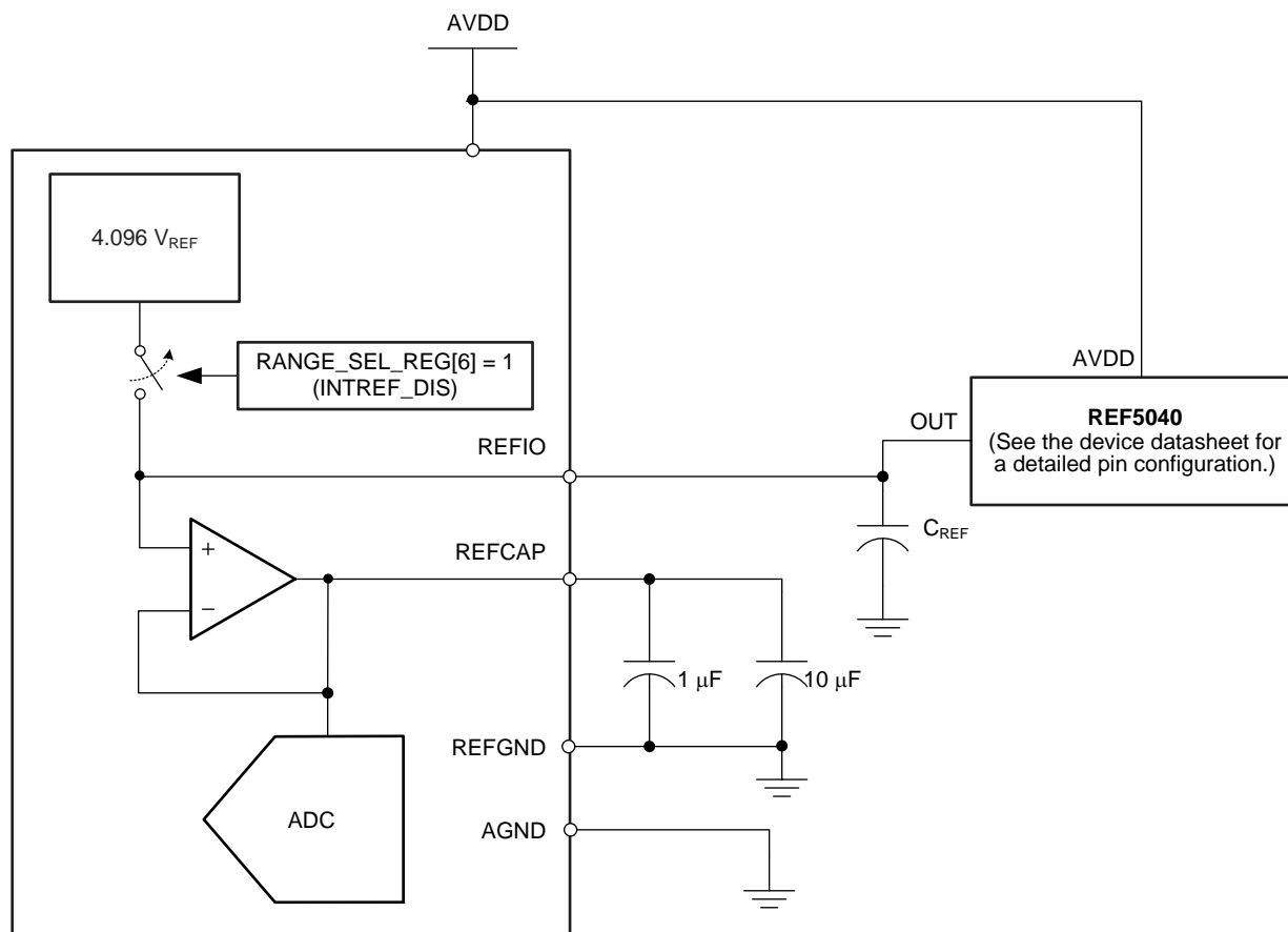
Figure 58. Device Connections for Using an External 4.096-V Reference
