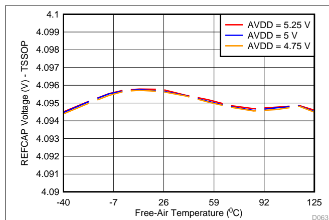
Figure 59. Reference Buffer Output (REFCAP) Variation vs Supply and Temperature
