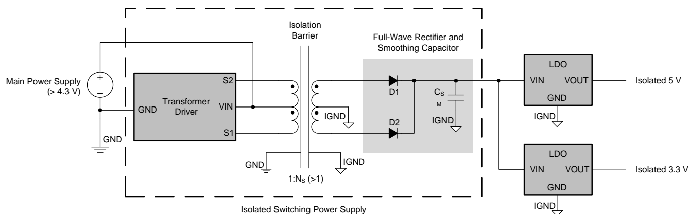
Figure 88. Isolated Power-Supply Design
