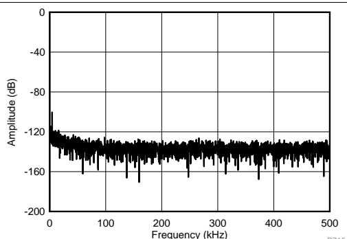
Figure 90. FFT Plot With an AC Common-Mode at 1 MSPS
