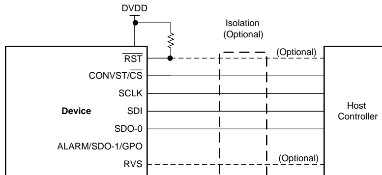
Figure 67. Standard SPI Protocol Pin Configuration
