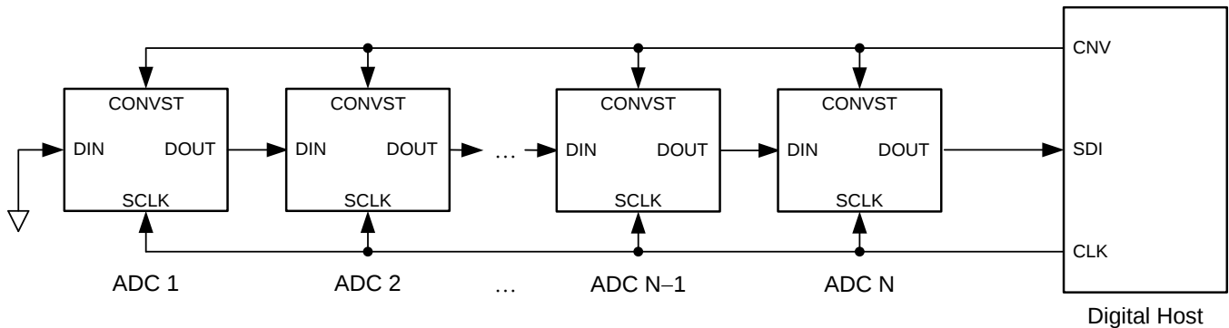
Figure 60. Connection Diagram: Daisy-Chain Mode Without a Busy Indicator ( \overline{\text{DIN}} = 0 )
