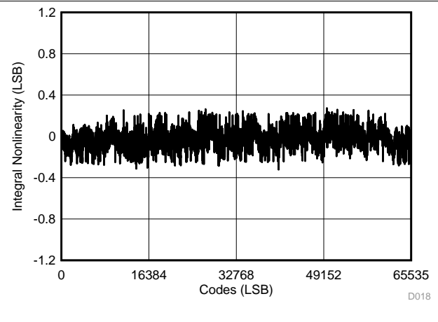
Figure 24. Typical INL for All Codes (All Bipolar Ranges)
